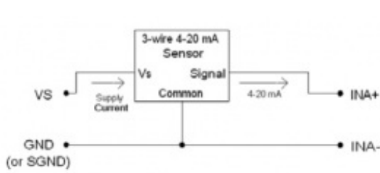
Figure 3: 3-Wire Sourcing Sensor
