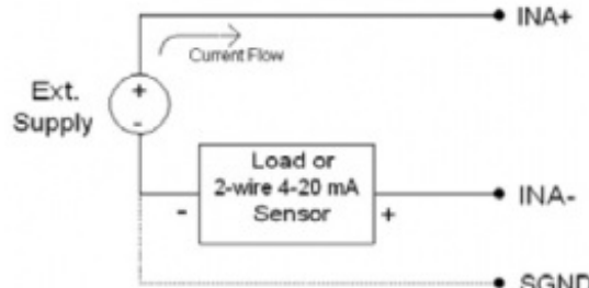
Figure 8: 2-Wire Sinking Sensor
